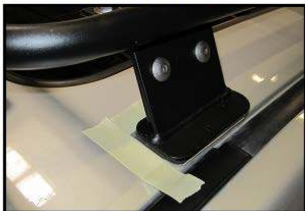
Fig. 18 Position both front driver and passenger side brackets as shown above and center roof rack on vehicle as shown in Fig. 19. Place masking tape as shown around the inside and front edges of support bracket.
